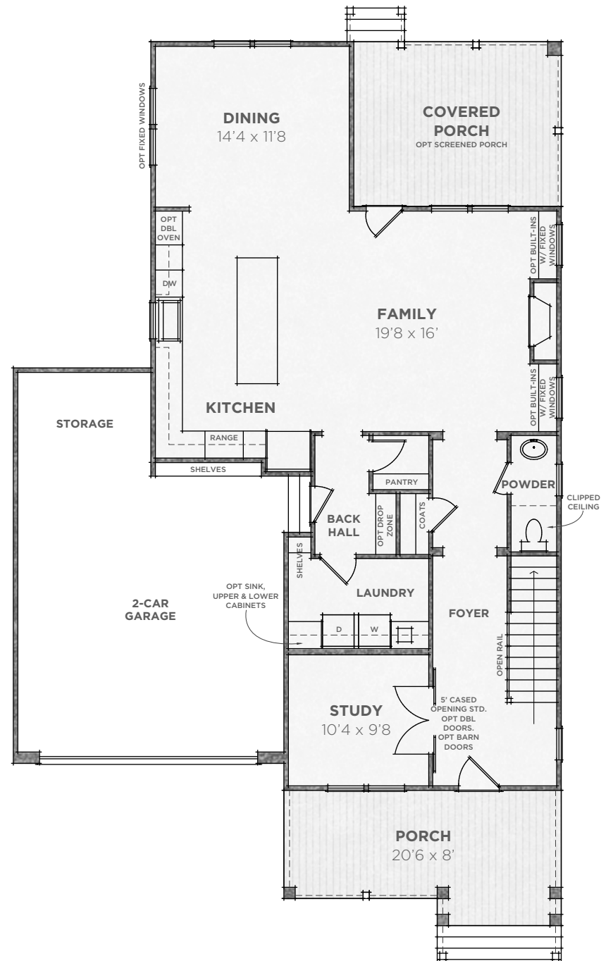
FIRST FLOOR
